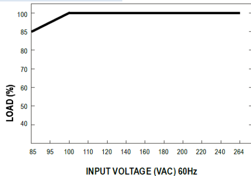
Static Characteristics
