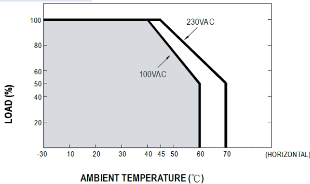
Derating Curve
