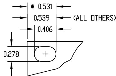
NOTCH DETAIL
