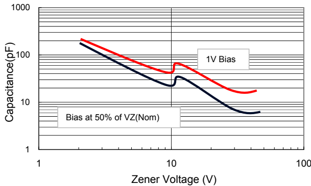
FIG 5 Typical Capacitance
