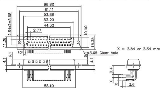
50 Positions Machined Pin (W/O Rear Cover)
