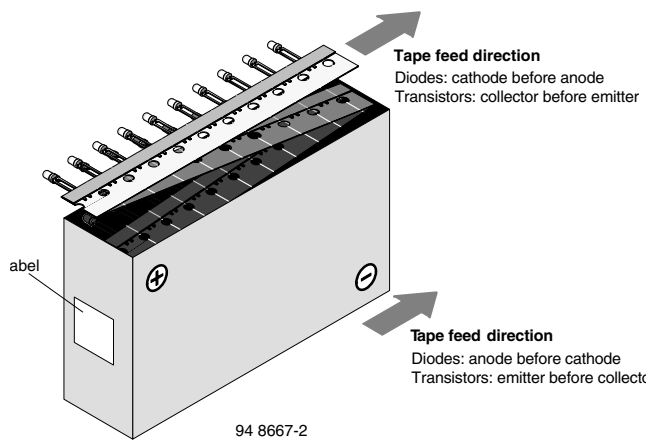
Fig. 20 - Tape Direction
