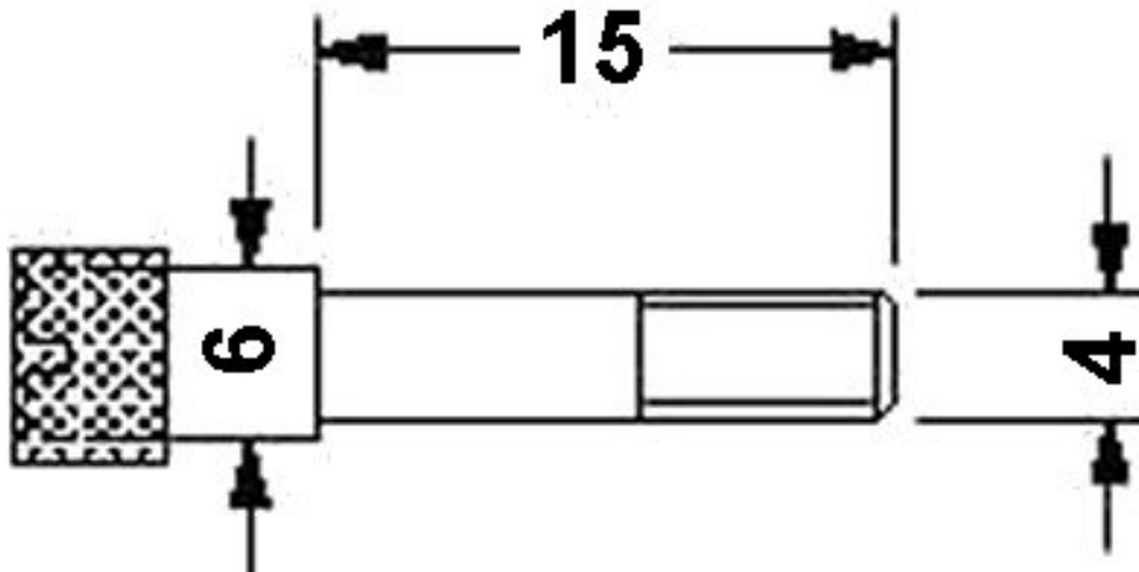
Dimensioned drawing
