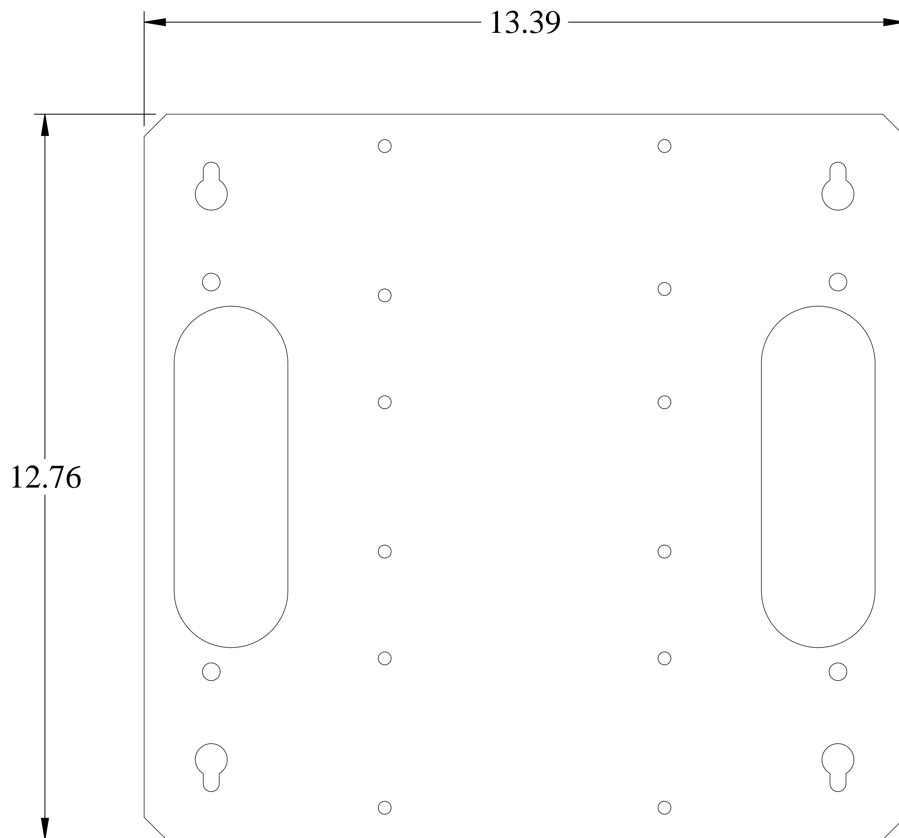
FRONT VIEW
