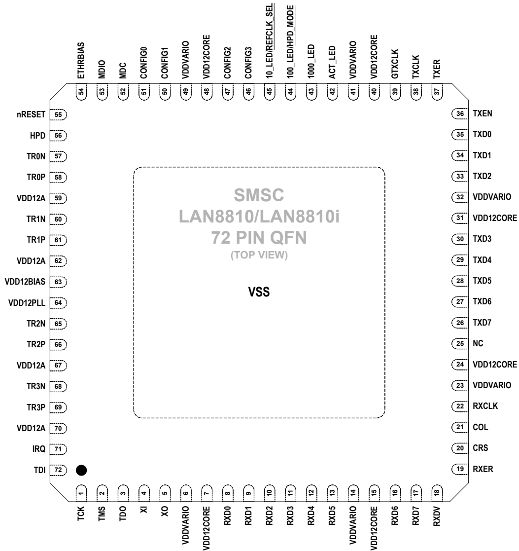
Figure 2.1 72-QFN Pin Assignments (TOP VIEW)
