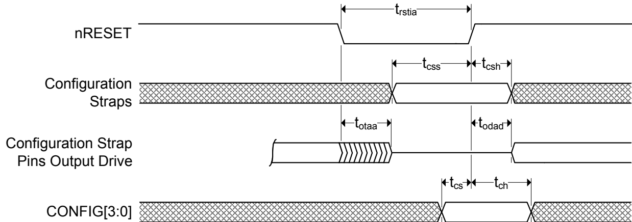
Figure 5.4 Reset Timing
